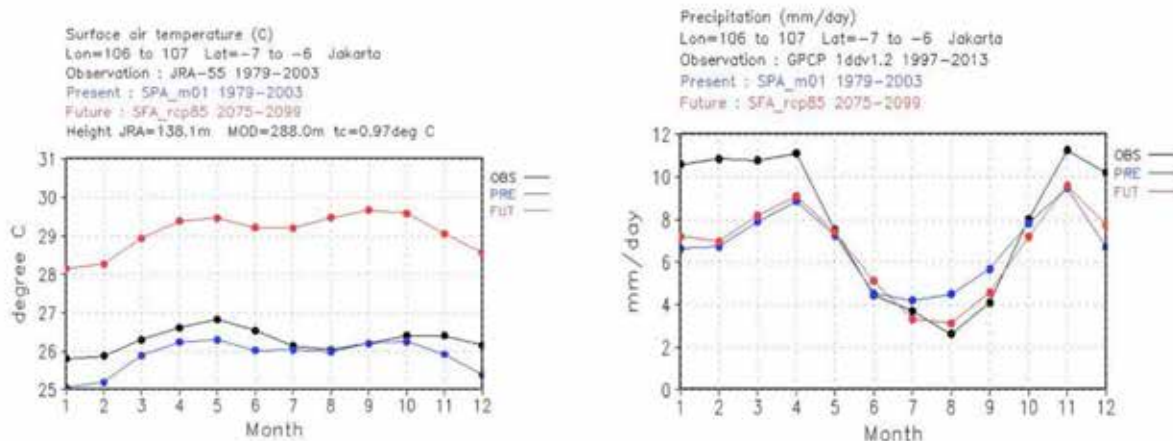
Fig. 3-3-1 Comparison of Temperature and Precipitation (Present and Future, Jakarta)
