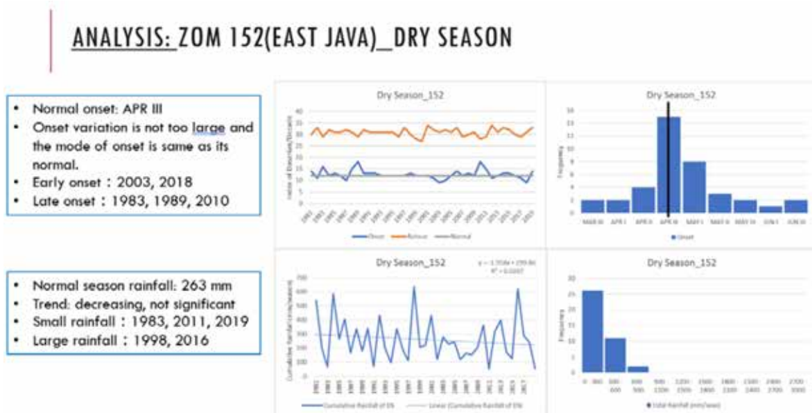
Fig. 3-2-10 Analysis of Dry Season Onset/Retreat Variability for ZOM152
