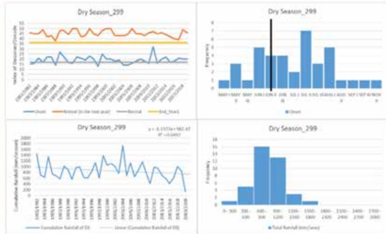
Fig. 3-2-13 Analysis of Dry Season Onset/Retreat Variability for ZOM299
