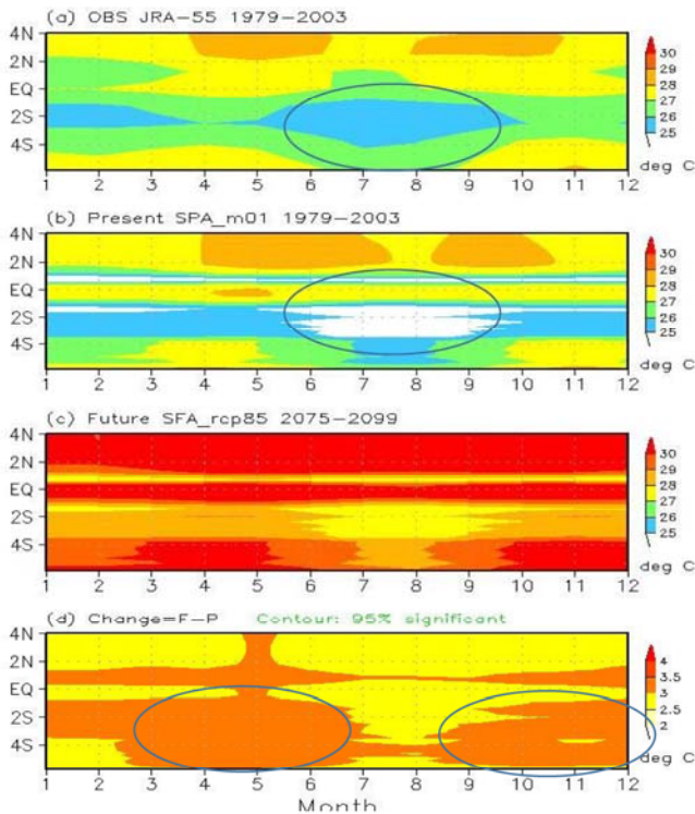
Surface air temperature (deg C) Lon=118 to 125.4 Month=1 to 12
