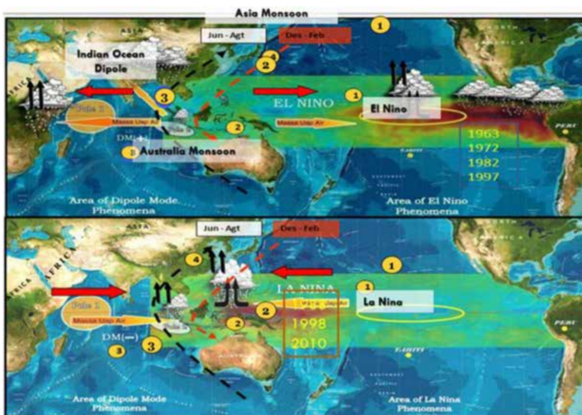
Fig. 3-2-1 Major Climatic Drivers in Indonesia (from BMKG)
