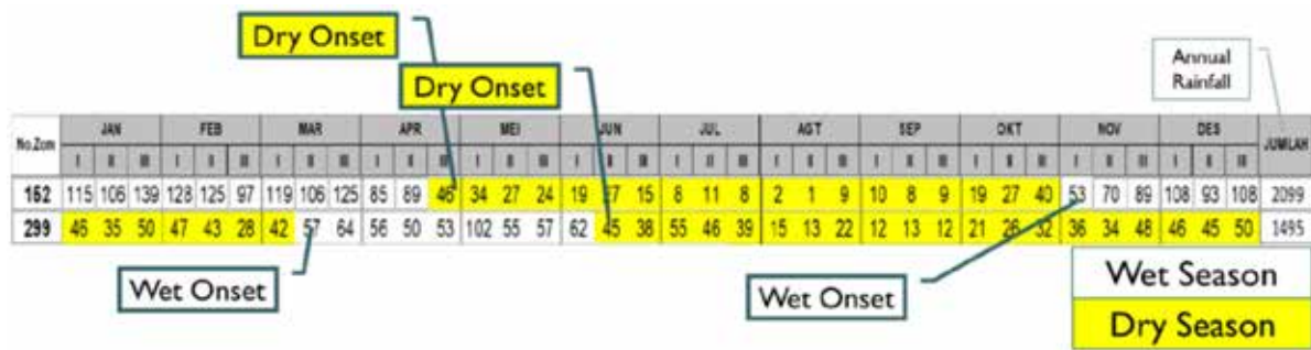
Figure 1-1-1. Determination of the start of the season based on BMKG criteria
