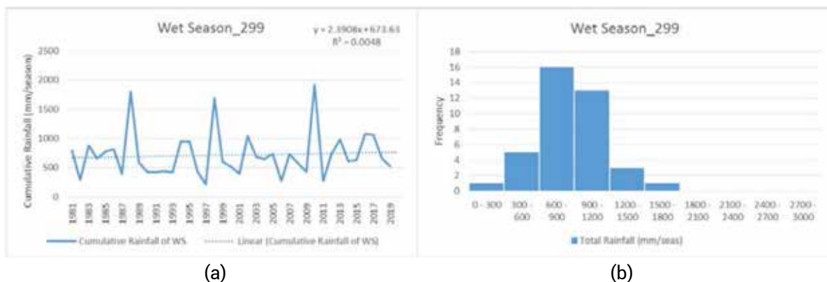
Figure 8. Trend (a) and distribution (b) of wet season's cumulative rainfall in ZOM 299
