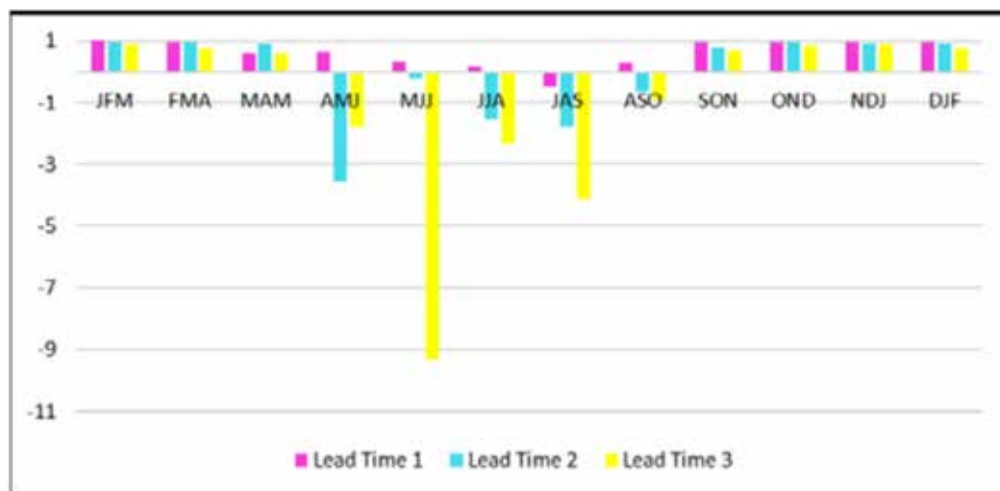
Fig. 3-2-22 Performance of Nino 3.4 Prediction Issued by NCEP using MSSS Method
