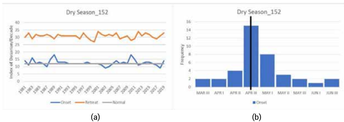
Figure 1-2-1 Variation (a) and distribution (b) of dry Season onset in ZOM 152 to its normal
