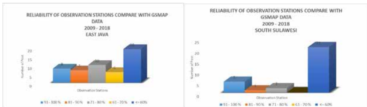
Figure 3-3-4. Reliability of GSMaP data compared to the ground observations
