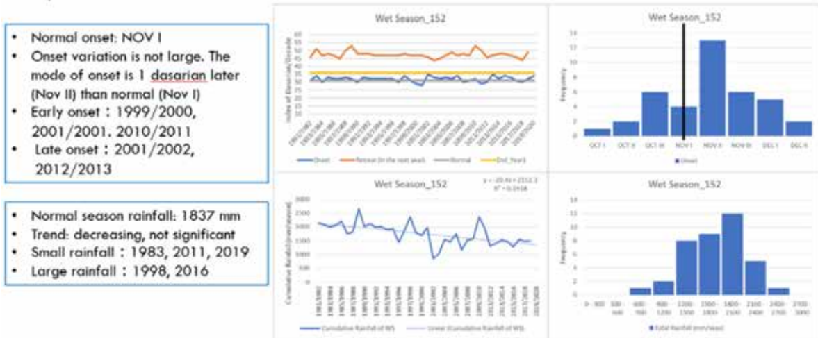
Fig. 3-2-11 Analysis of Wet Season Onset/Retreat Variability for ZOM152
